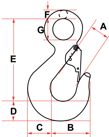
STANDARD HOOK WITH SAFETY LATCH
