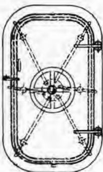
#104 6-DOG QUICK ACTING DOOR
