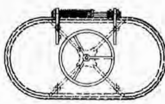
#215 SPRING BALANCED OVAL QUICK ACTING HATCH
