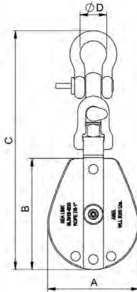
DRILLED SWIVEL EYE W/ SHACKLE (DS)
