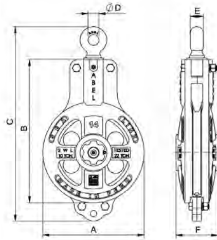
DRILLED SWIVEL EYE (DS)
